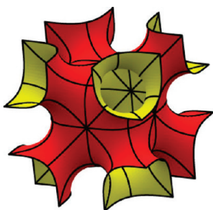
Figure 3. IW-P surface, posited as the structural element for the nanostructure of GMO-templated films after UV/O 3 treatment or acid extraction. Yellow and red signify interior volumes with 8-fold and 4-fold connectivity, respectively.
