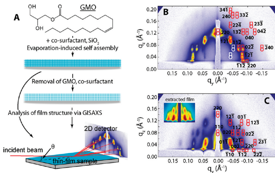
Figure 1. (A) Structure of GMO and general procedure for fabrication and analysis of nanoporous films using this template and (B) and (C) GISAXS data for GMO/ diC 6 PC-templated silica films. (B) As deposited, indexed to space group Ia3d (double gyroid). Circles and squares indicate the predicted positions of scattering arising from the direct and reflected beams, respectively. White signifies the position of normally forbidden reflections for this space group. (C) After removal of the template by UV/O 3 treatment, indexed to space group Im3m . The inset contains GISAXS data for an acid-extracted film, also showing an Im3m nanostructure.
